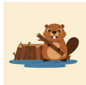
beaver
