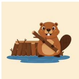
beaver
