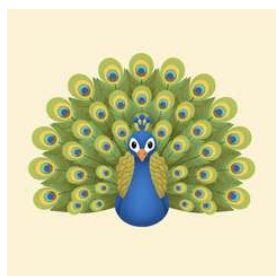
peacock
