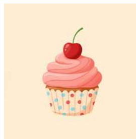
cupcake
