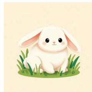
bunny
